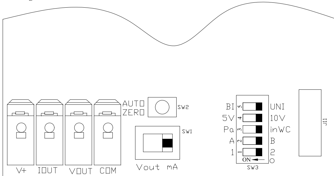
Figure 8: PCB Layout
