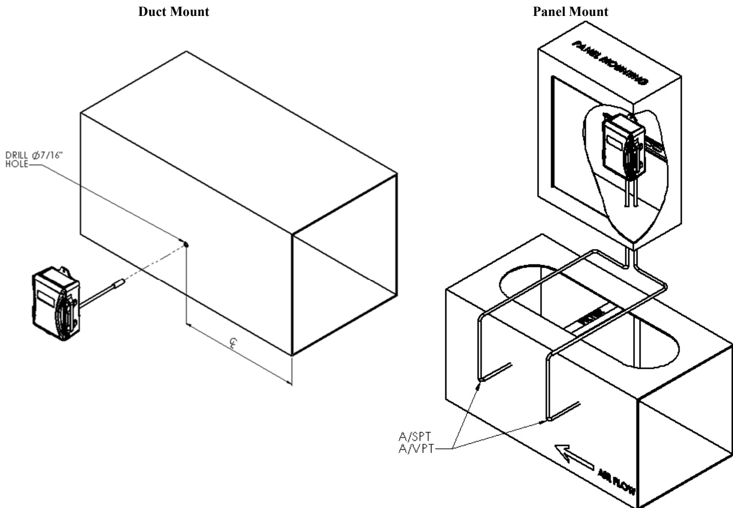
Figure 5: DLP Mounting
